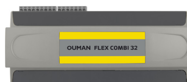
Measurements: width 213,5 mm (13M), height 90 mm, depth 93,3 mm
